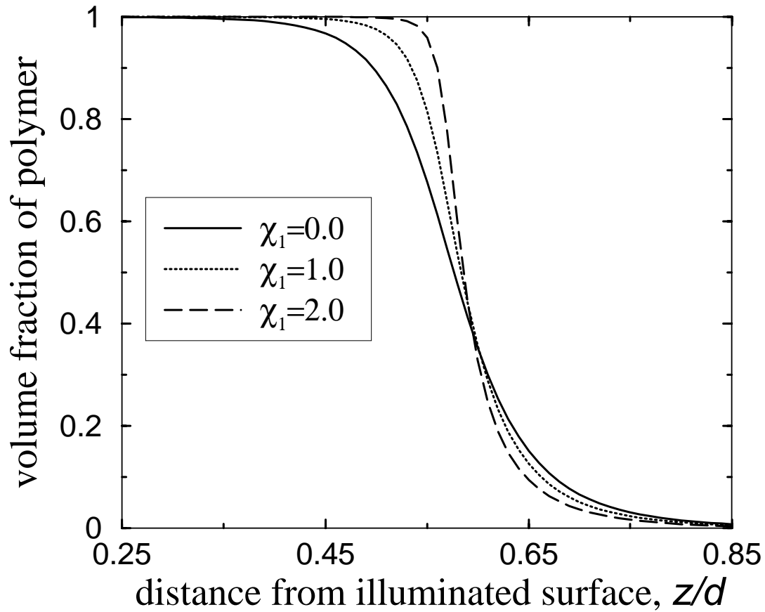
FIG. 6. Final volume fractions of polymer, which show better separation for larger \chi_1 . The parameters used for calculation are \phi_0/\psi_0 = 60/40 , L = 0.05 , R = 0.05 , and \chi_1 = 0, 1.0 and 2.0 .
