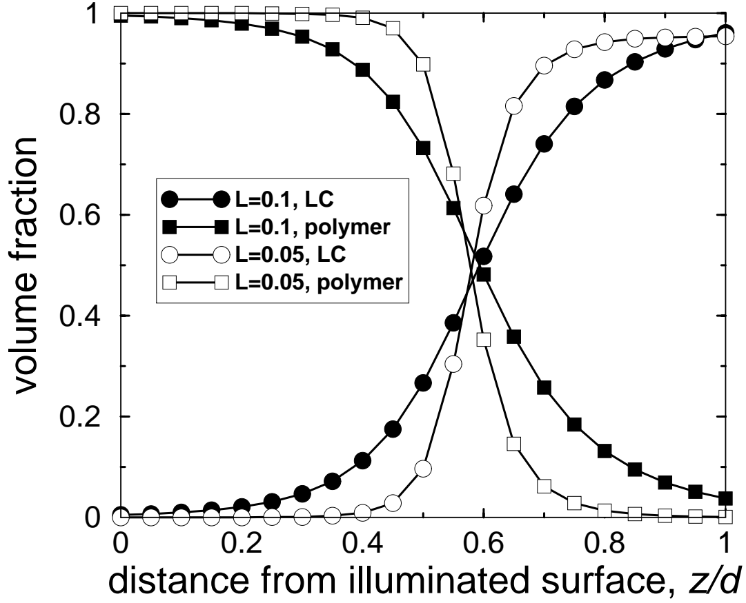
FIG. 3. Final volume fractions of LC and polymer, which show better separation for shorter absorption length of light. The parameters used for calculation are \phi_0/\psi_0 = 60/40 , L = 0.10 and 0.05 , R = 0.05 , and \chi_1 = 0 .
