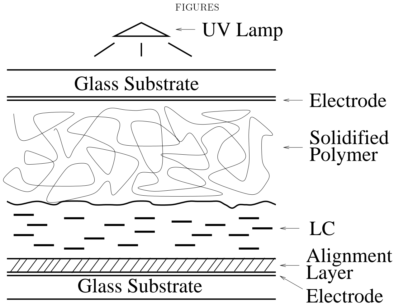
FIG. 1. Schematic of the PSCOF structure
