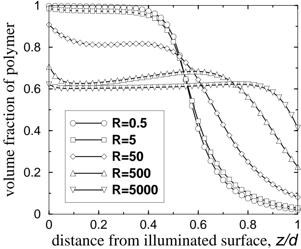
FIG. 4. Final volume fraction of polymer, which shows better separation for slower polymerization. The parameters used for calculation are \phi_0/\psi_0 = 60/40 , L = 0.10 , R = 0.5, 5, 50, 500 , and 5000 , and \chi_1 = 2.0 .
