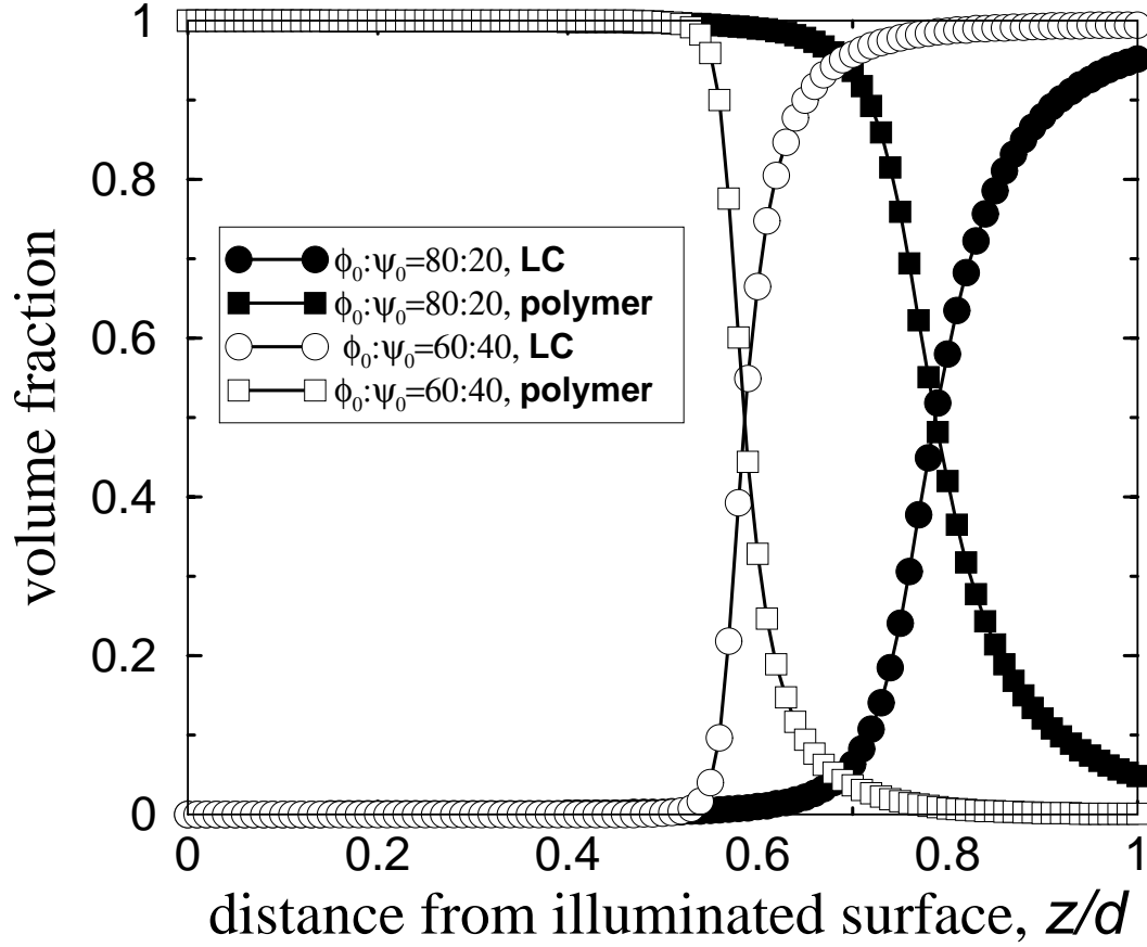
FIG. 5. Final volume fractions of LC and polymer, which show better separation for more equal initial volume fractions of prepolymer and LC. The parameters used for calculation are \phi_0/\psi_0 = 80/20 and 60/40 , L = 0.05 , R = 0.05 , and \chi_1 = 2.0 .
